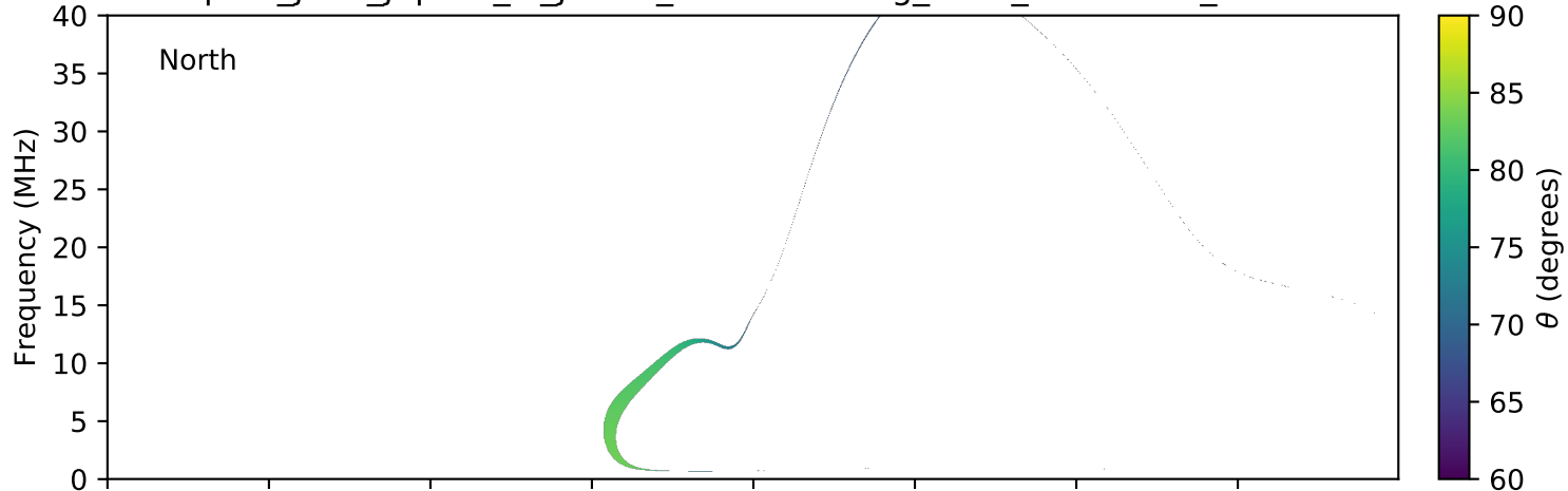
expres_juno_jupiter_io_jrm09_lossc-wid1deg_3kev_20160605_v01.cdf
