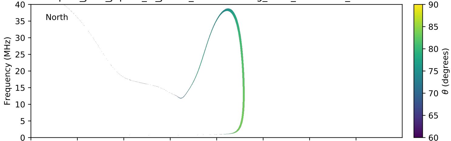
expres_juno_jupiter_io_jrm09_lossc-wid1deg_3kev_20160604_v01.cdf
