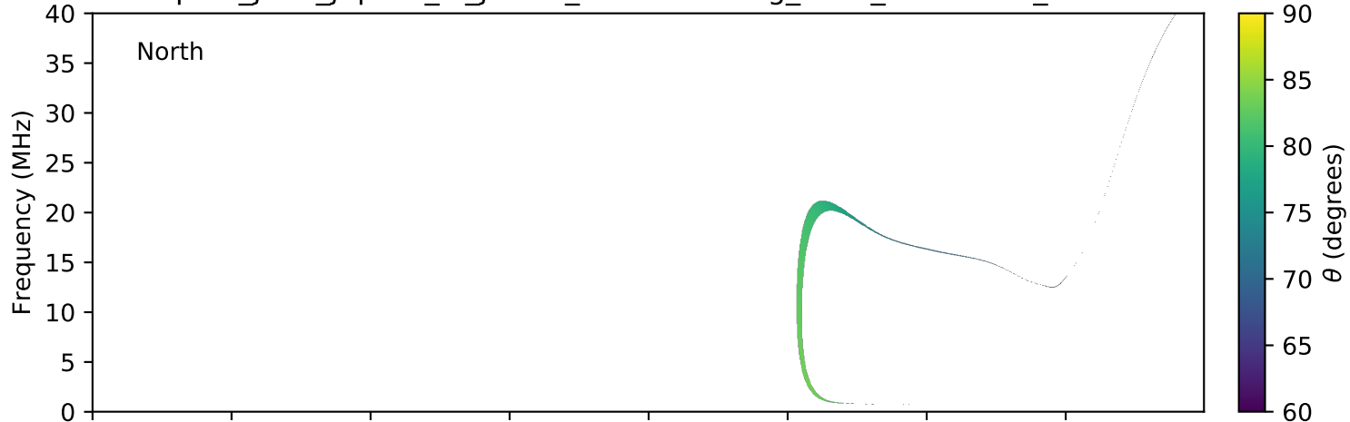
expres_juno_jupiter_io_jrm09_lossc-wid1deg_3kev_20160603_v01.cdf
