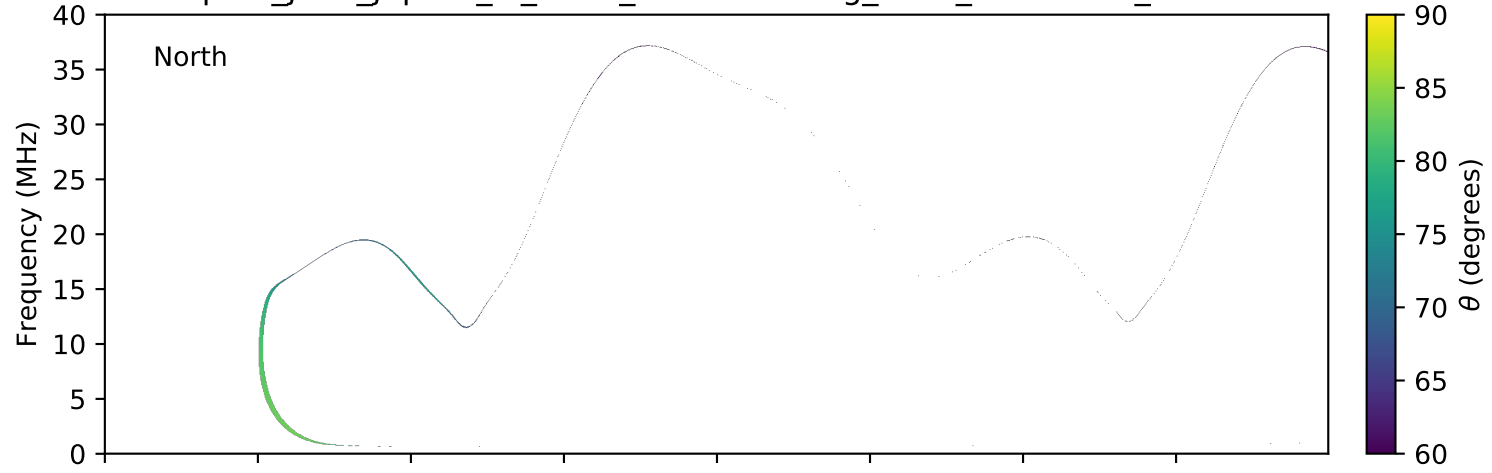
expres_juno_jupiter_io_isaac_lossc-wid1deg_3kev_20160630_v01.cdf
