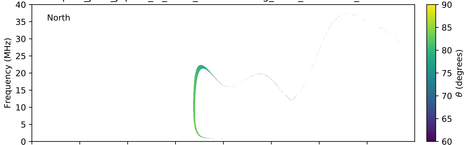
expres_juno_jupiter_io_isaac_lossc-wid1deg_3kev_20160628_v01.cdf
