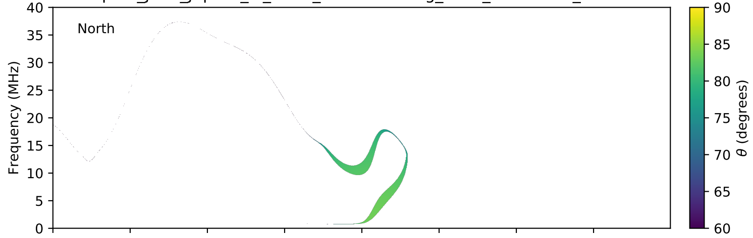
expres_juno_jupiter_io_isaac_lossc-wid1deg_3kev_20160627_v01.cdf
