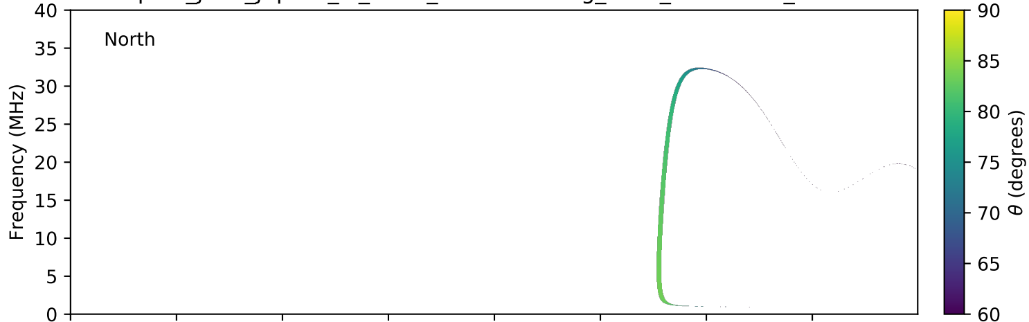
expres_juno_jupiter_io_isaac_lossc-wid1deg_3kev_20160626_v01.cdf
