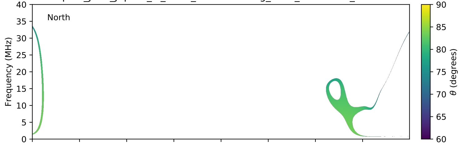
expres_juno_jupiter_io_isaac_lossc-wid1deg_3kev_20160624_v01.cdf
