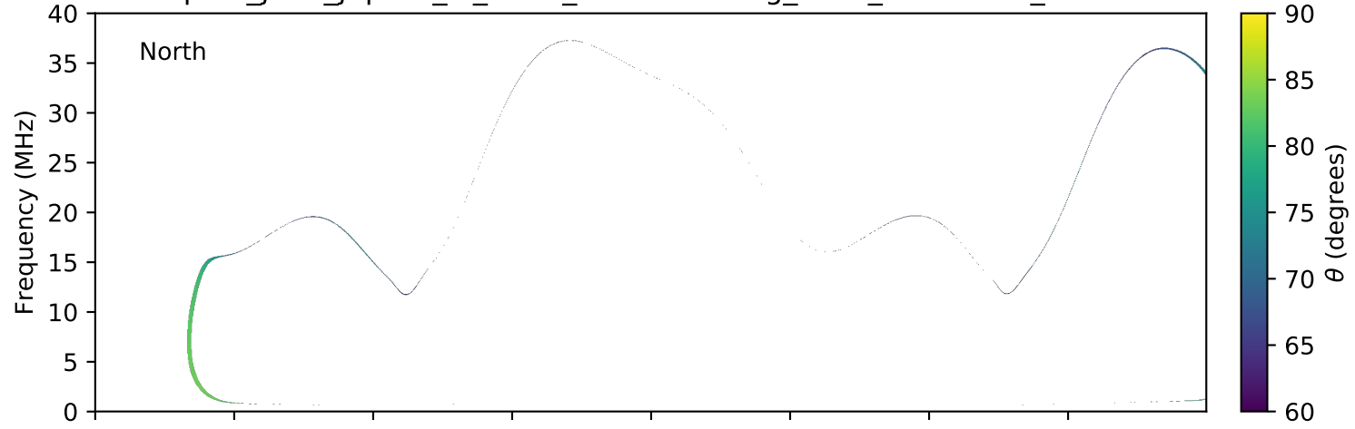
expres_juno_jupiter_io_isaac_lossc-wid1deg_3kev_20160623_v01.cdf
