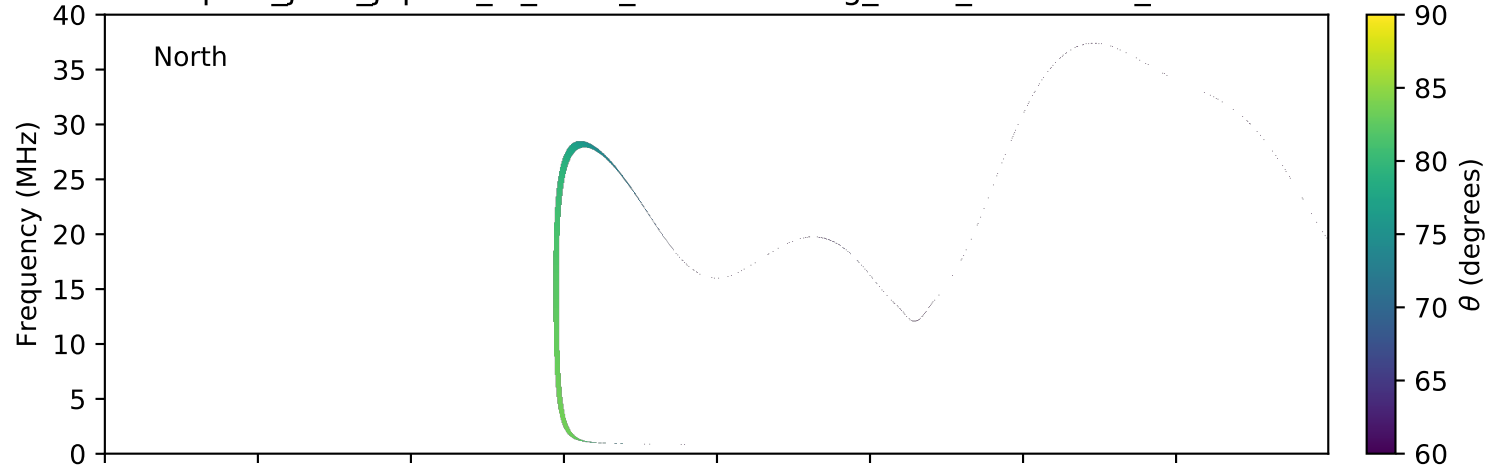
expres_juno_jupiter_io_isaac_lossc-wid1deg_3kev_20160621_v01.cdf
