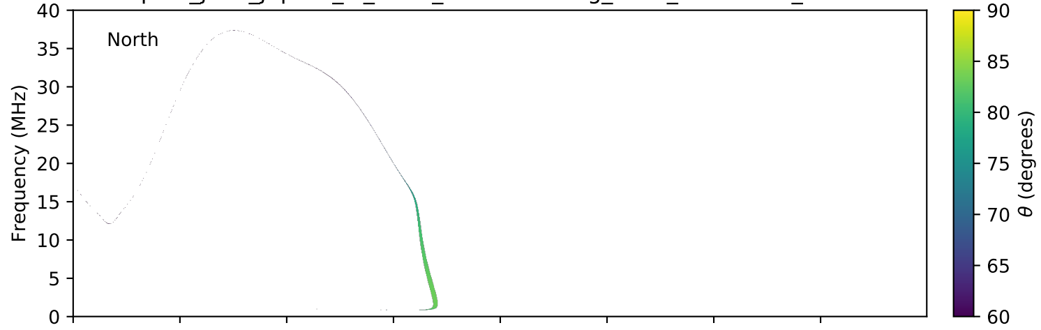
expres_juno_jupiter_io_isaac_lossc-wid1deg_3kev_20160620_v01.cdf
