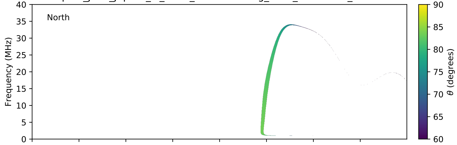
expres_juno_jupiter_io_isaac_lossc-wid1deg_3kev_20160619_v01.cdf
