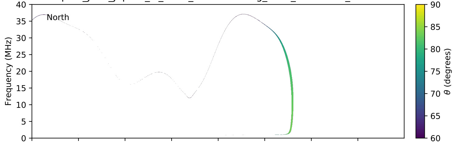
expres_juno_jupiter_io_isaac_lossc-wid1deg_3kev_20160618_v01.cdf
