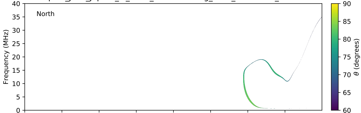
expres_juno_jupiter_io_isaac_lossc-wid1deg_3kev_20160617_v01.cdf
