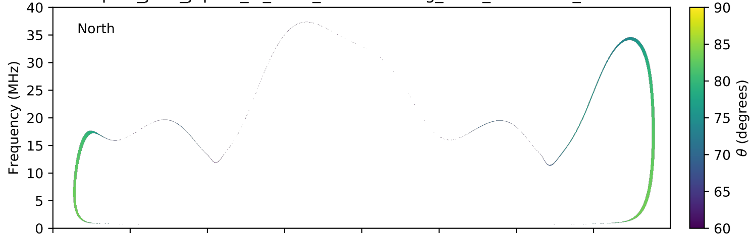
expres_juno_jupiter_io_isaac_lossc-wid1deg_3kev_20160616_v01.cdf
