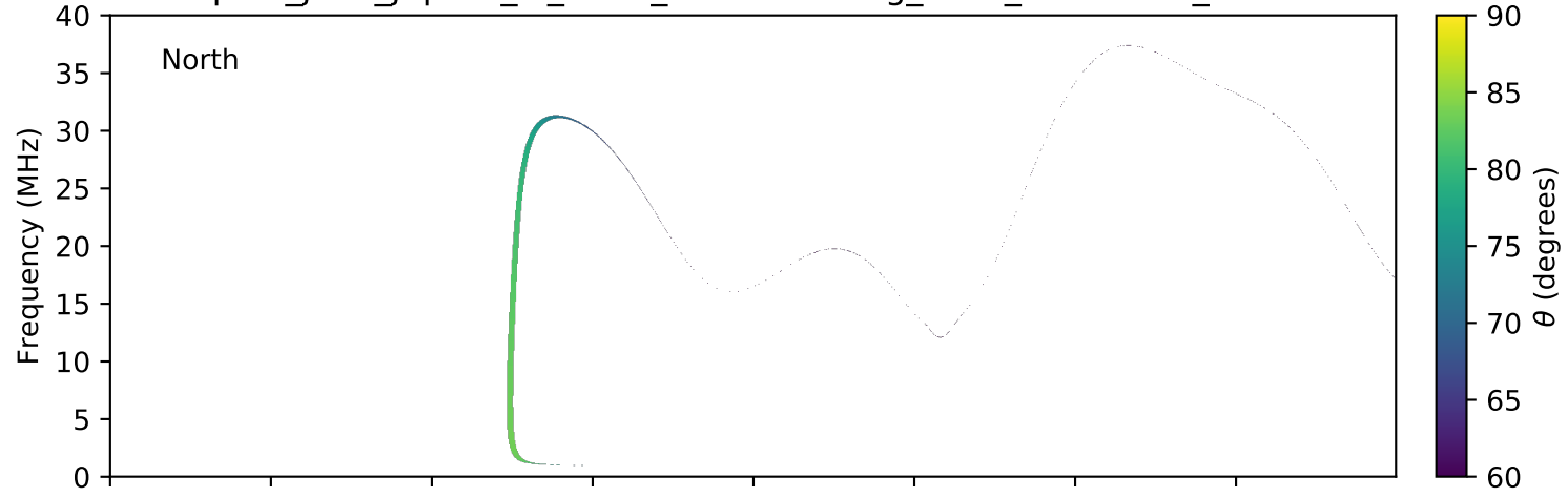
expres_juno_jupiter_io_isaac_lossc-wid1deg_3kev_20160614_v01.cdf
