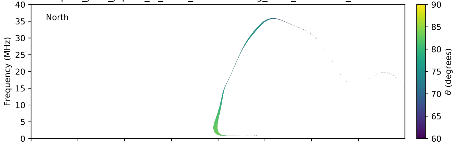
expres_juno_jupiter_io_isaac_lossc-wid1deg_3kev_20160612_v01.cdf
