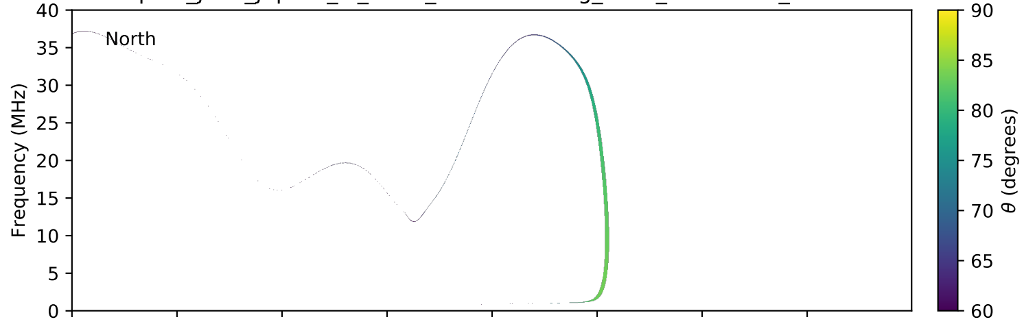
expres_juno_jupiter_io_isaac_lossc-wid1deg_3kev_20160611_v01.cdf
