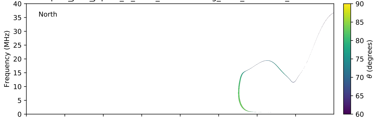
expres_juno_jupiter_io_isaac_lossc-wid1deg_3kev_20160610_v01.cdf
