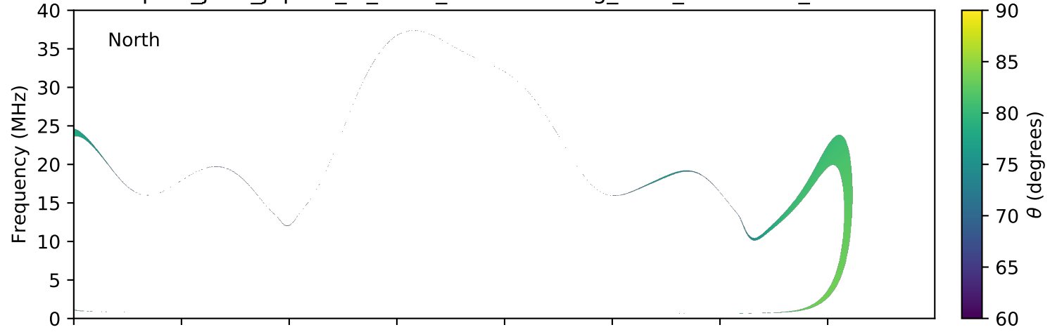
expres_juno_jupiter_io_isaac_lossc-wid1deg_3kev_20160609_v01.cdf
