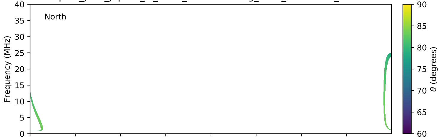
expres_juno_jupiter_io_isaac_lossc-wid1deg_3kev_20160608_v01.cdf
