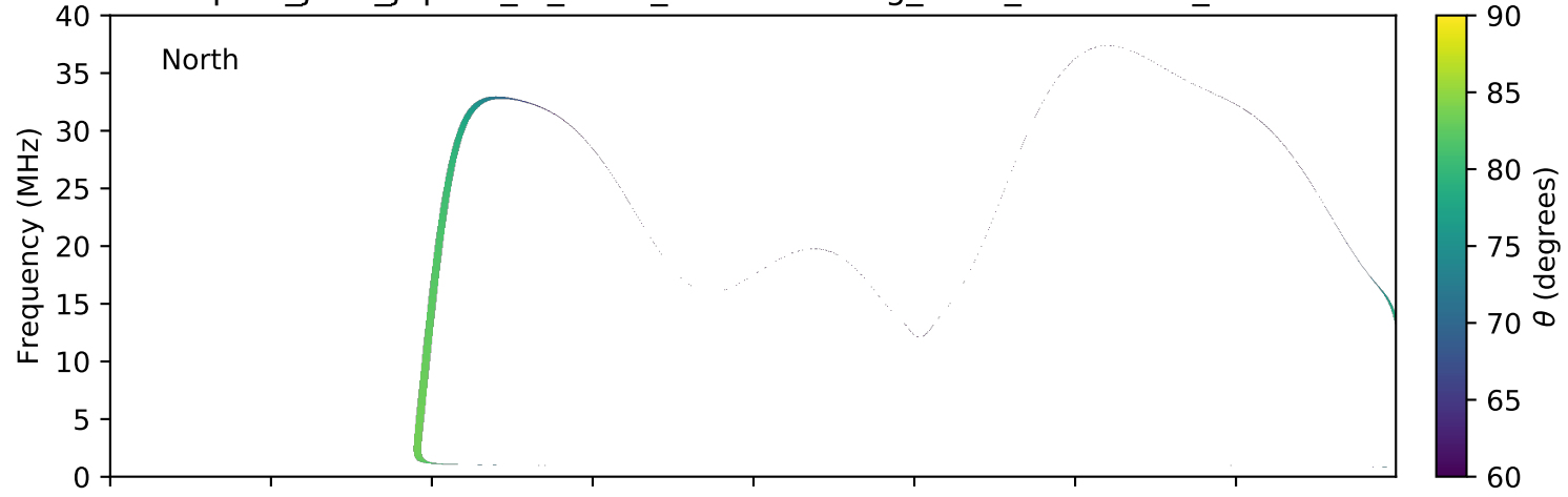
expres_juno_jupiter_io_isaac_lossc-wid1deg_3kev_20160607_v01.cdf
