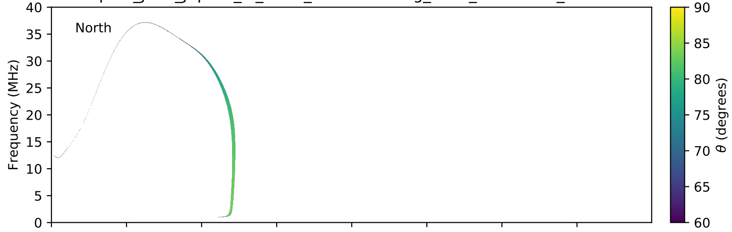
expres_juno_jupiter_io_isaac_lossc-wid1deg_3kev_20160606_v01.cdf
