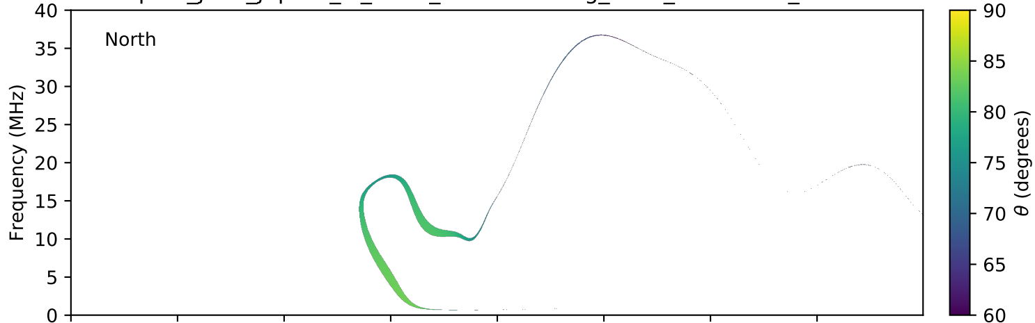
expres_juno_jupiter_io_isaac_lossc-wid1deg_3kev_20160605_v01.cdf
