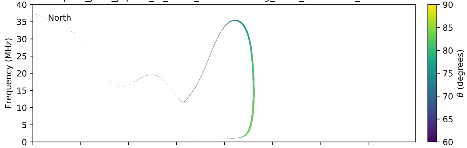
expres_juno_jupiter_io_isaac_lossc-wid1deg_3kev_20160604_v01.cdf
