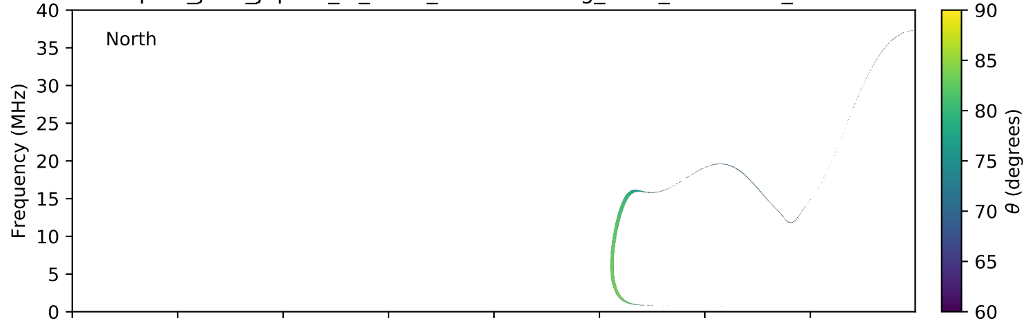
expres_juno_jupiter_io_isaac_lossc-wid1deg_3kev_20160603_v01.cdf
