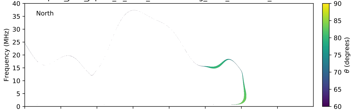
expres_juno_jupiter_io_isaac_lossc-wid1deg_3kev_20160602_v01.cdf
