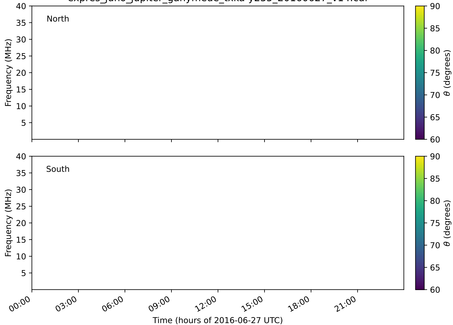
expres_juno_jupiter_ganymede_txka-y235_20160627_v14.cdf
