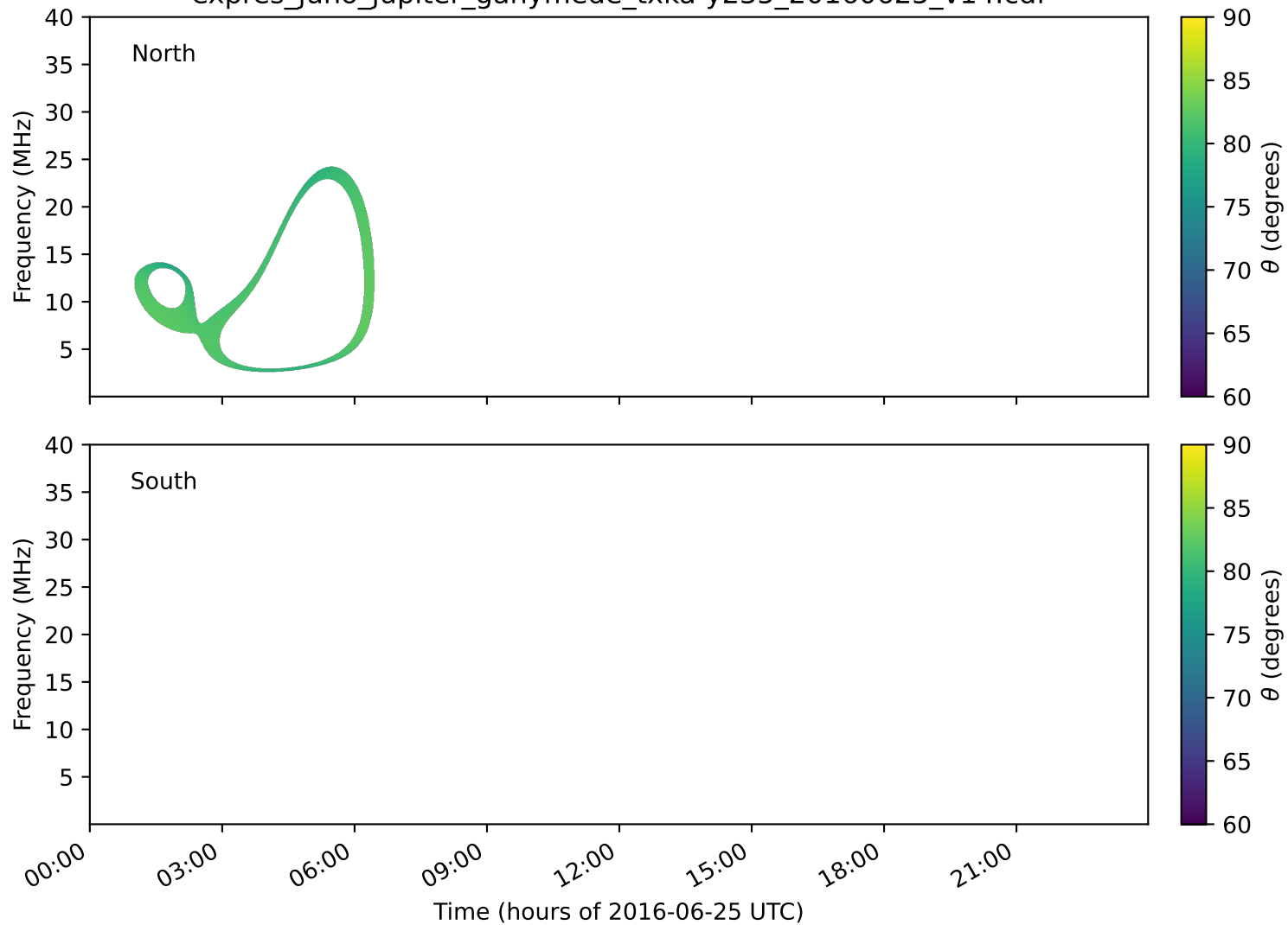
expres_juno_jupiter_ganymede_txka-y235_20160625_v14.cdf
