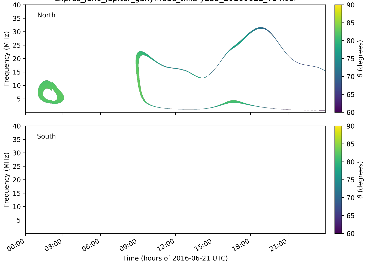
expres_juno_jupiter_ganymede_txka-y235_20160621_v14.cdf
