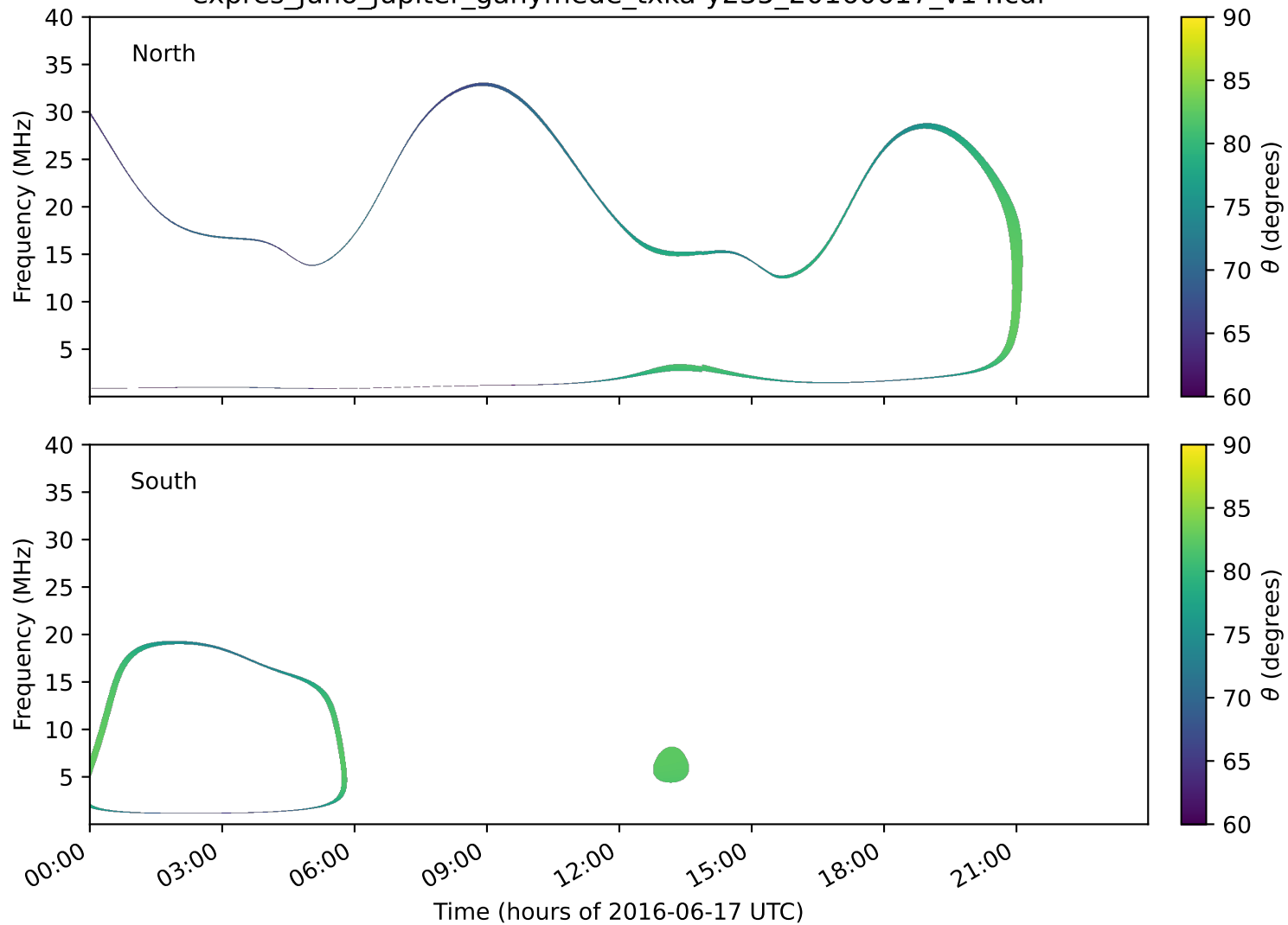
expres_juno_jupiter_ganymede_txka-y235_20160617_v14.cdf
