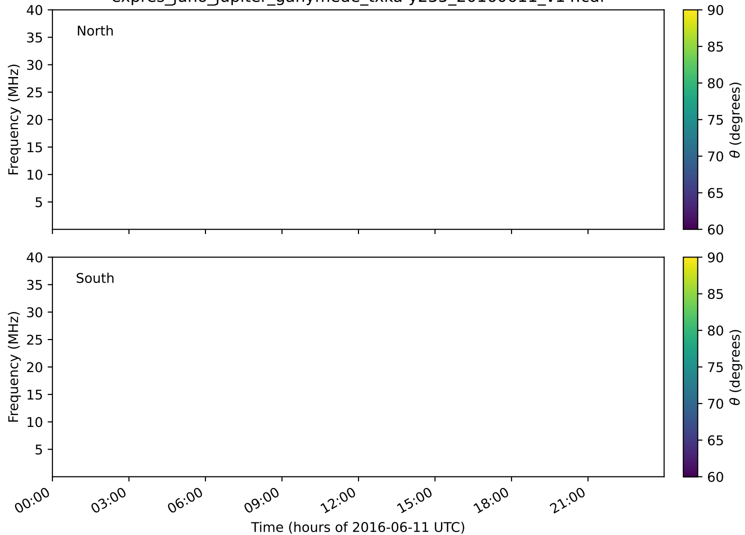
expres_juno_jupiter_ganymede_txka-y235_20160611_v14.cdf
