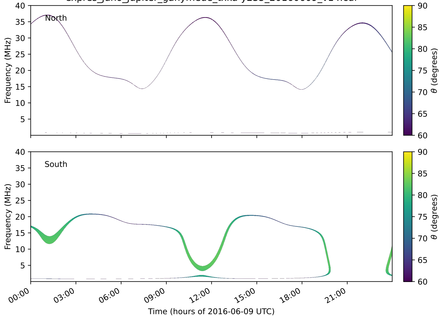
expres_juno_jupiter_ganymede_txka-y235_20160609_v14.cdf
