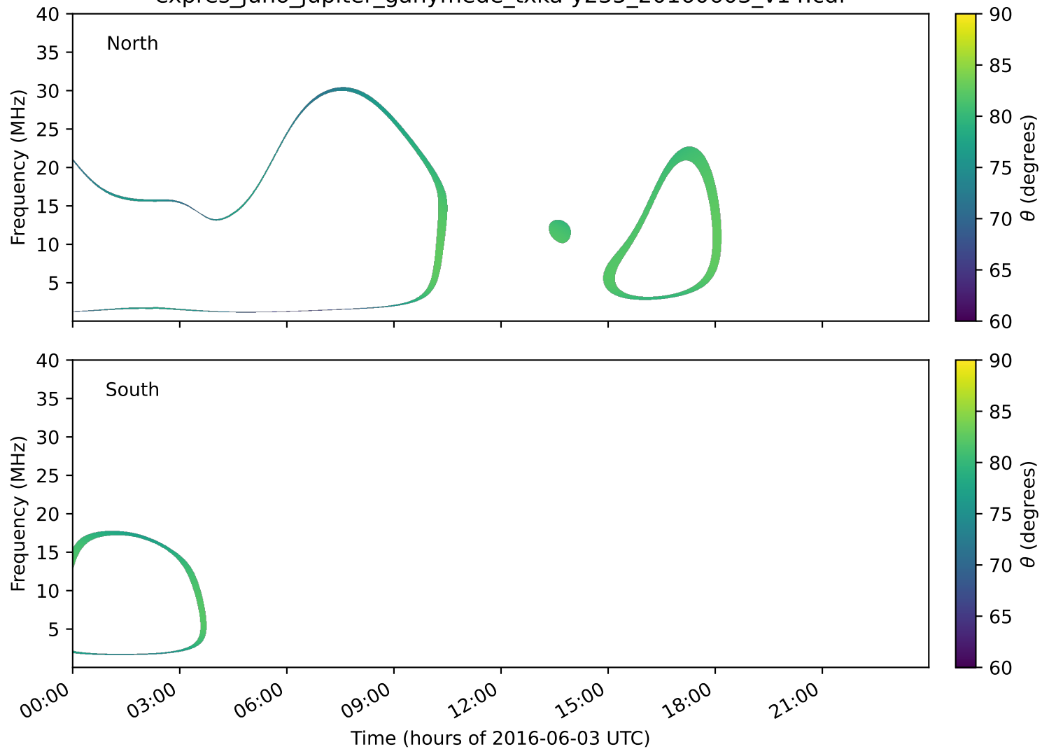
expres_juno_jupiter_ganymede_txka-y235_20160603_v14.cdf
