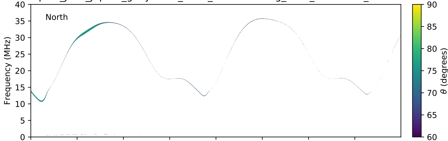
expres_juno_jupiter_ganymede_isaac_lossc-wid1deg_3kev_20160629_v01.cdf
