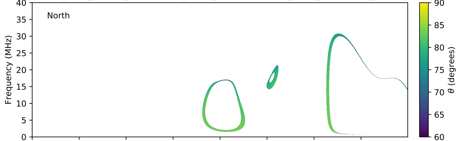
expres_juno_jupiter_ganymede_isaac_lossc-wid1deg_3kev_20160628_v01.cdf
