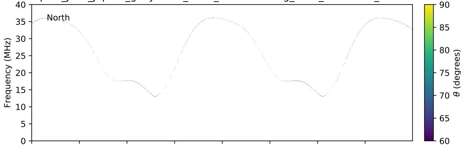
expres_juno_jupiter_ganymede_isaac_lossc-wid1deg_3kev_20160623_v01.cdf
