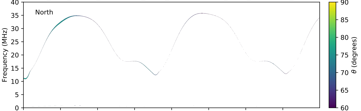
expres_juno_jupiter_ganymede_isaac_lossc-wid1deg_3kev_20160622_v01.cdf
