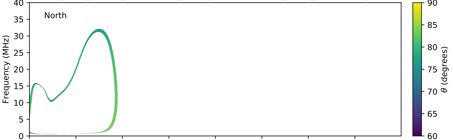
expres_juno_jupiter_ganymede_isaac_lossc-wid1deg_3kev_20160618_v01.cdf
