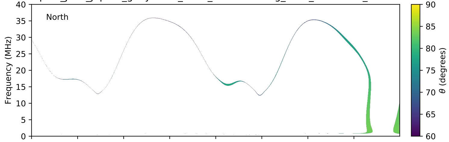
expres_juno_jupiter_ganymede_isaac_lossc-wid1deg_3kev_20160617_v01.cdf
