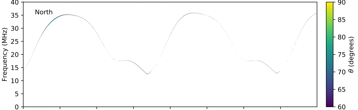
expres_juno_jupiter_ganymede_isaac_lossc-wid1deg_3kev_20160615_v01.cdf
