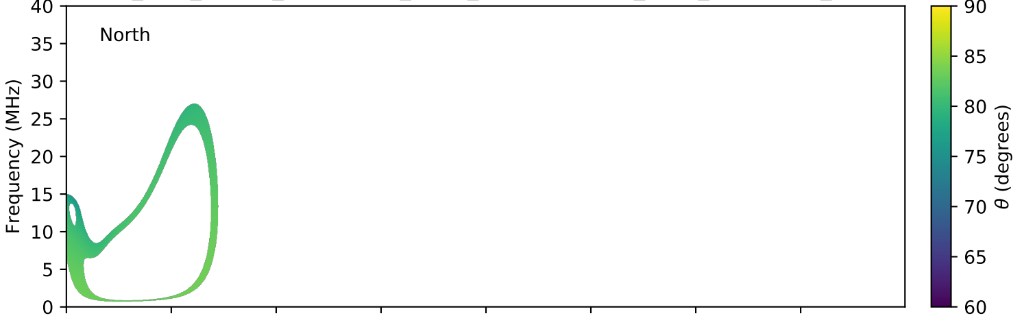
expres_juno_jupiter_ganymede_isaac_lossc-wid1deg_3kev_20160611_v01.cdf
