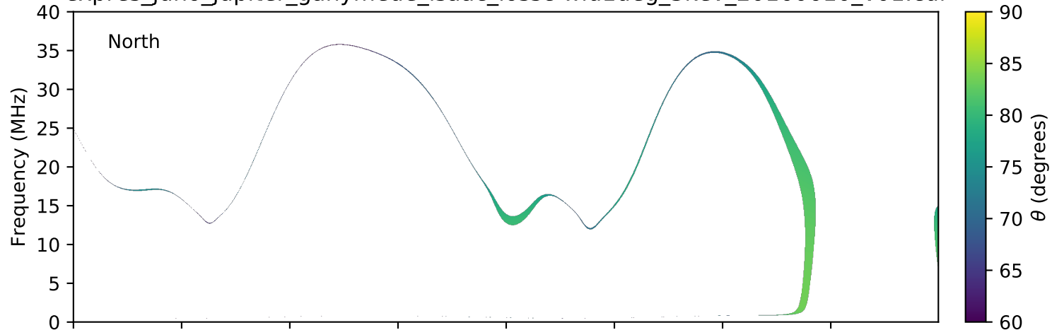
expres_juno_jupiter_ganymede_isaac_lossc-wid1deg_3kev_20160610_v01.cdf
