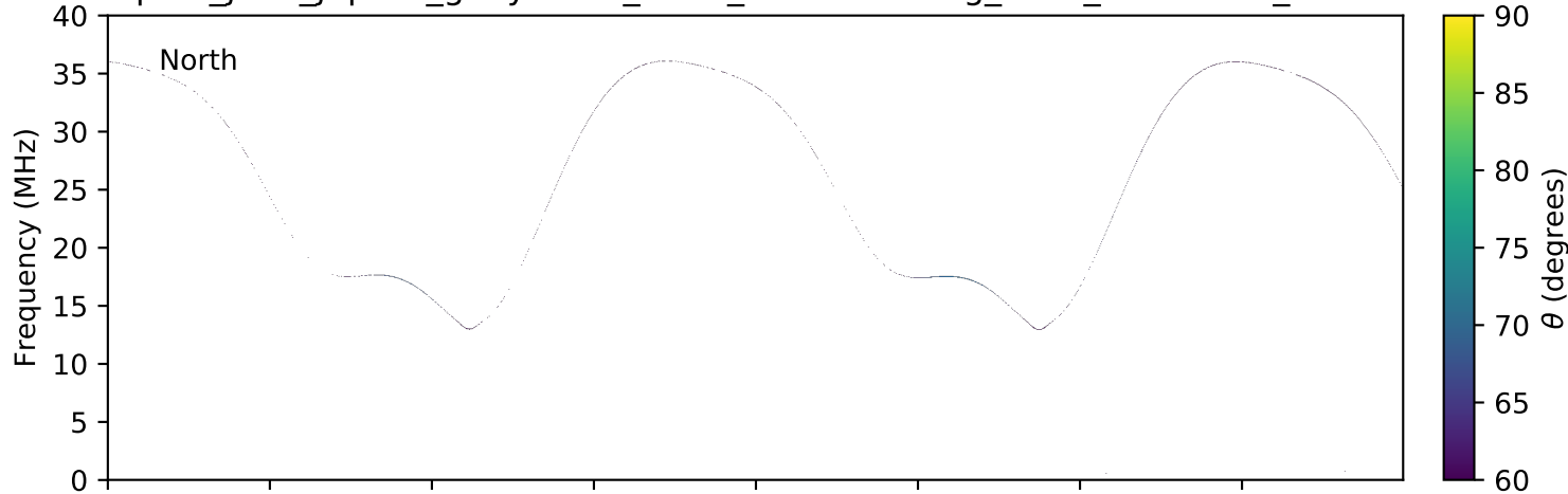
expres_juno_jupiter_ganymede_isaac_lossc-wid1deg_3kev_20160609_v01.cdf
