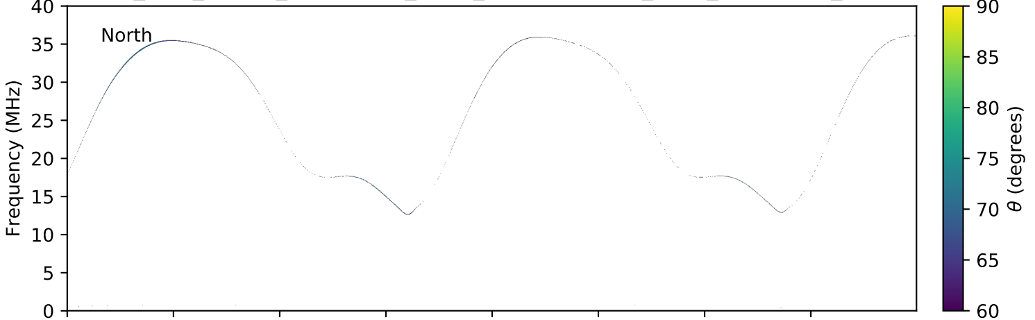
expres_juno_jupiter_ganymede_isaac_lossc-wid1deg_3kev_20160608_v01.cdf
