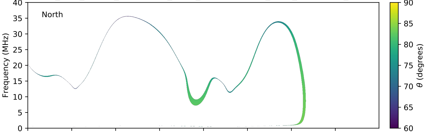
expres_juno_jupiter_ganymede_isaac_lossc-wid1deg_3kev_20160603_v01.cdf
