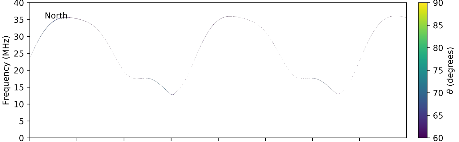
expres_juno_jupiter_ganymede_isaac_lossc-wid1deg_3kev_20160601_v01.cdf
