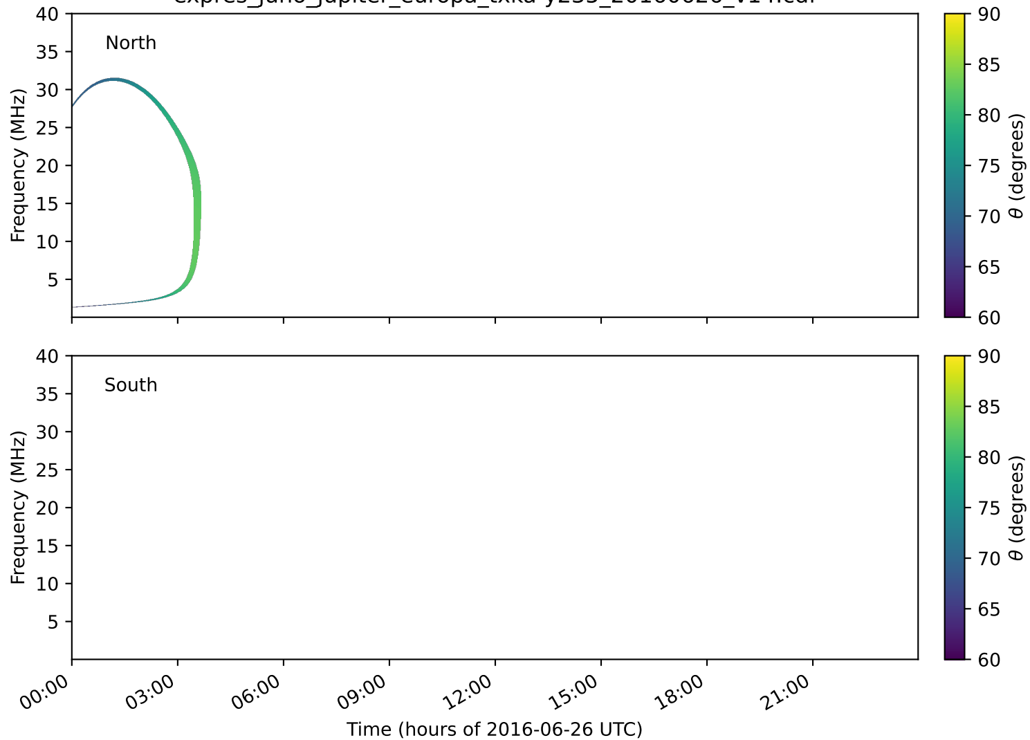
expres_juno_jupiter_europa_txka-y235_20160626_v14.cdf
