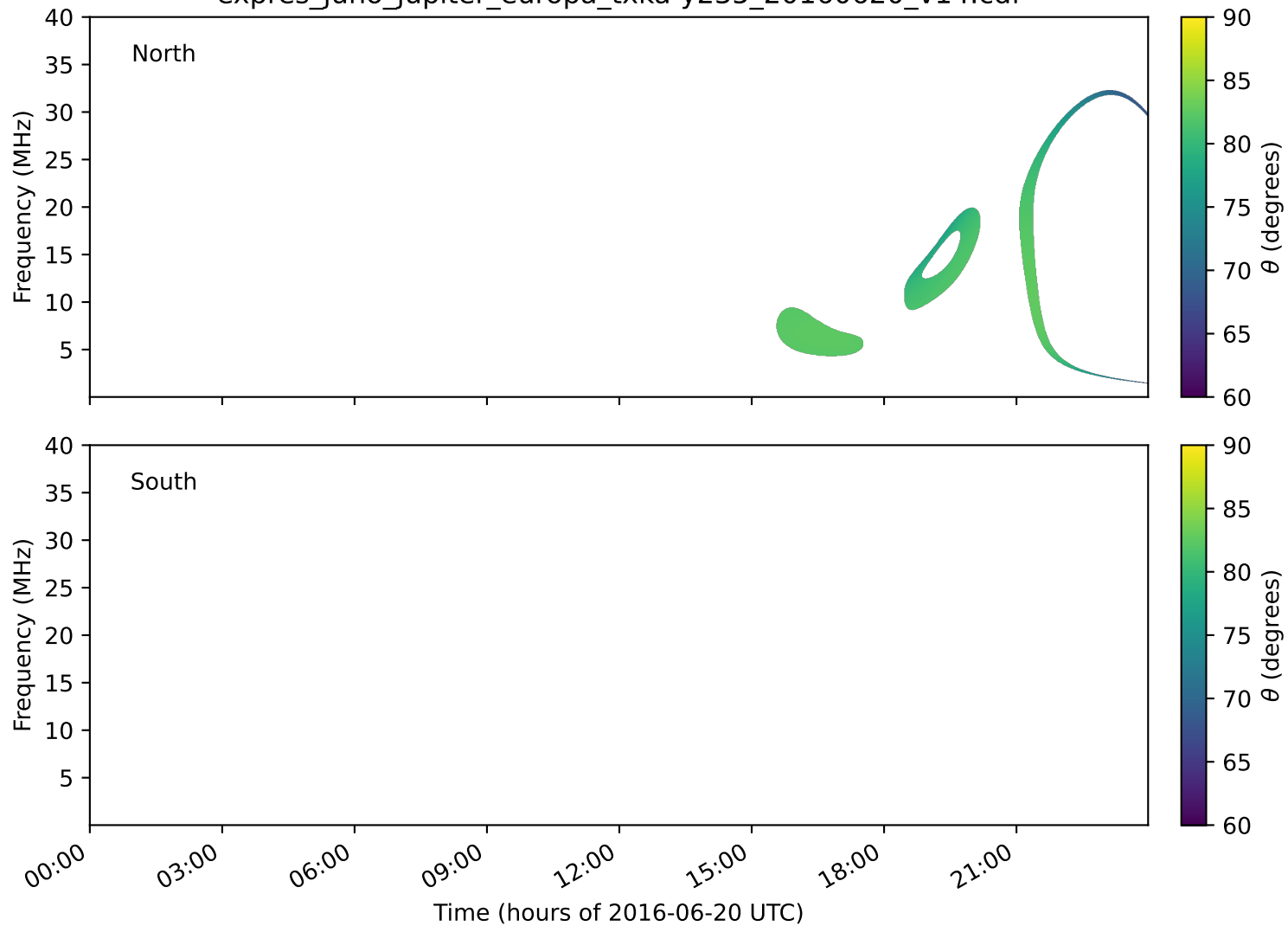
expres_juno_jupiter_europa_txka-y235_20160620_v14.cdf
