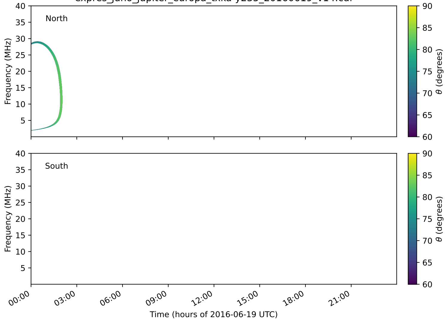
expres_juno_jupiter_europa_txka-y235_20160619_v14.cdf
